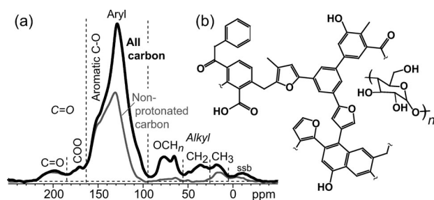
Figure 5. a) Quantitative ^{13}\text{C} NMR spectra of all carbon atoms (thick line), and of nonprotonated carbon atoms and \text{CH}_3 groups (thin line) in ^{13}\text{C} -enriched carbon-SBA-15, ssb = spinning sideband (14 kHz MAS); b) structural model reproducing the experimental spectra.
